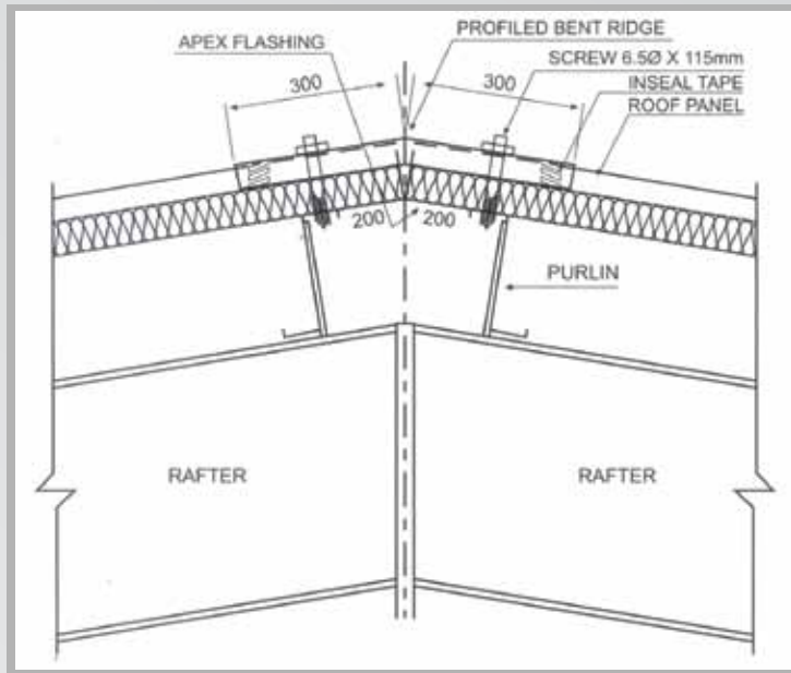
SANDWICH PANEL
